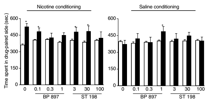
Figure 1 BP 897 (D 3 R partial agonist) and ST 198 (D 3 R antagonist) inhibit the expression of nicotine CPPs. The figures represent the time spent in seconds (+ SEM) in the initially less-preferred side of the apparatus during pre-conditioning (open bar) and post-conditioning (closed bar) 900-s sessions. All the animals received three pairings of either nicotine (0.1 mg/kg, left panel) or saline (right panel). On the test day, animals received either saline ( n = 19 – 21 ), BP 897 ( n = 14 – 16 , i.p.) or ST 198 ( 12 – 14 , p.o.) 30 min after being placed into the CPP apparatus and the time spent in each chamber was automatically recorded for 900 s. * P < 0.05 as compared to saline-treated rats the test day.
